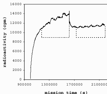
Figure 4: LR data from Viking Lander 2, test cycle 1, with two segments indicated by dashed brackets. The sharp transition in LR in the middle marks the second administration of radiolabeled nutrients.
